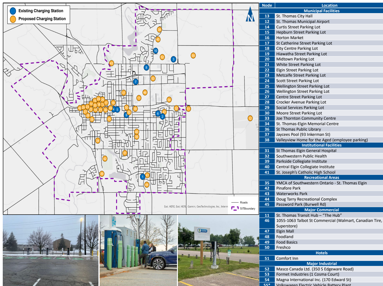
FIGURE 6.3: RECOMMENDED ELECTRIC VEHICLE CHARGING NETWORK
