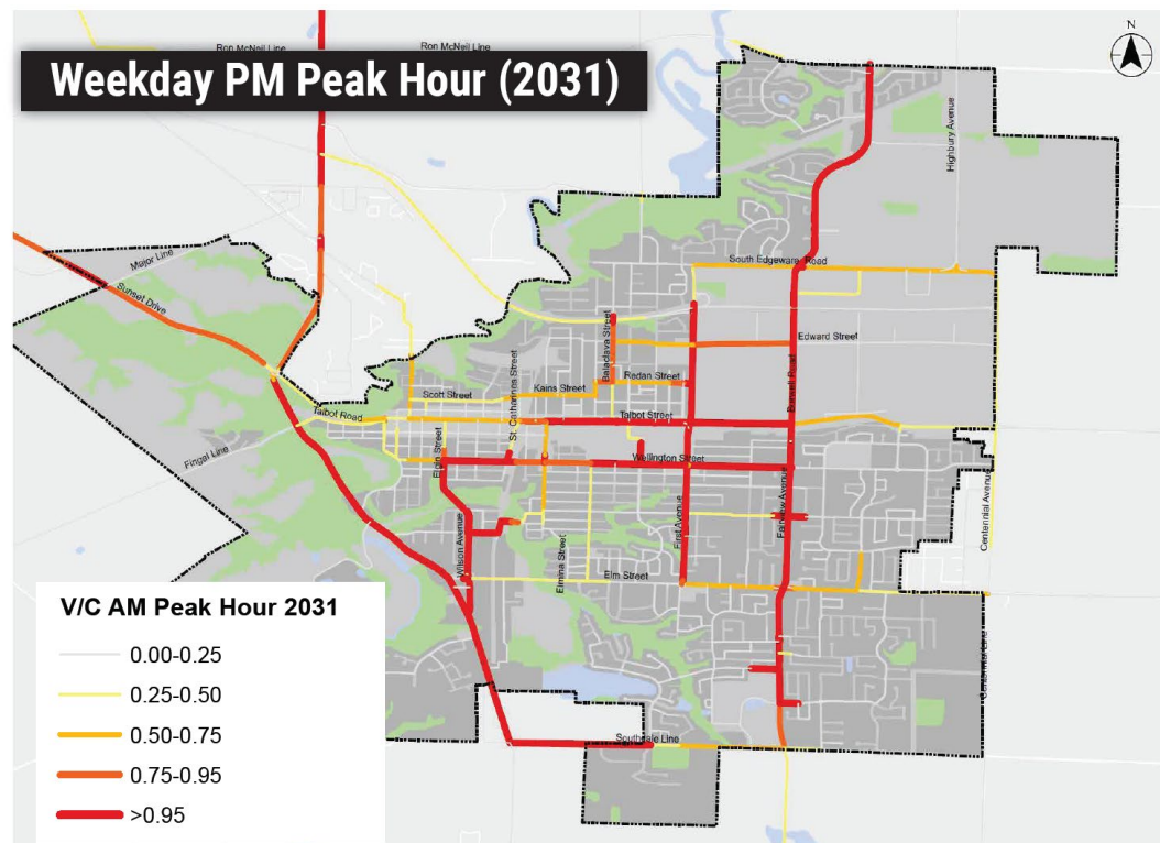
Figure 3.5: Forecasted growth operational analysis | Weekday PM Peak period
