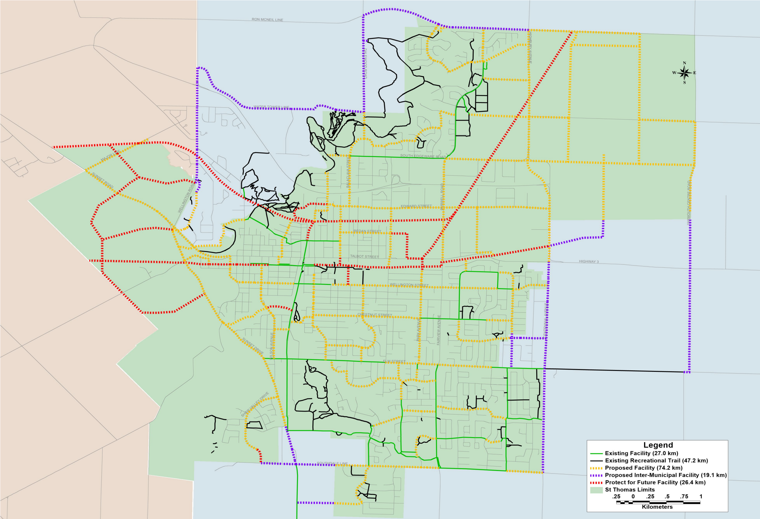
FIGURE 5.8: RECOMMENDED ACTIVE TRANSPORTATION NETWORK
