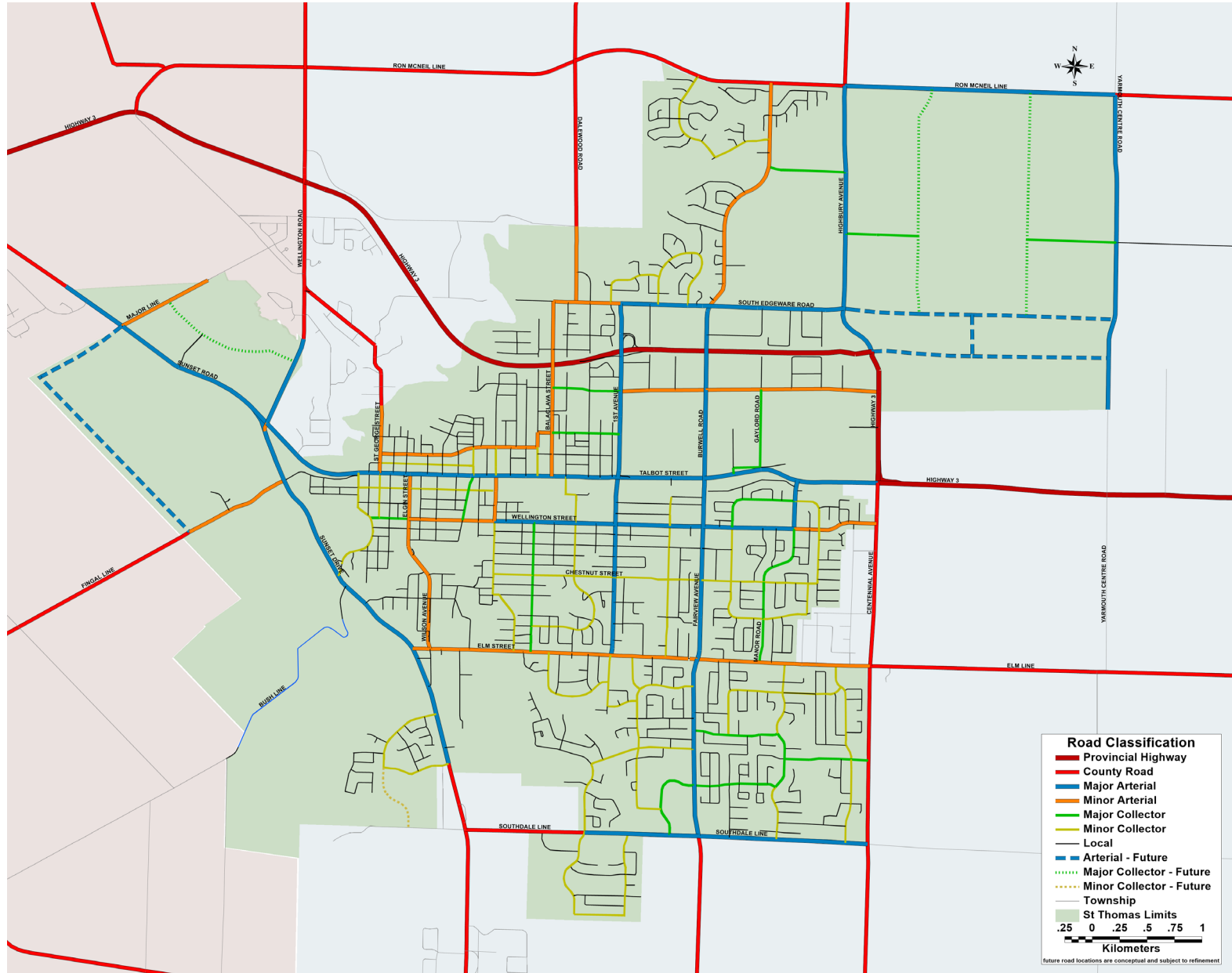
FIGURE 5.14: RECOMMENDED ROAD NETWORK CLASSIFICATIONS
