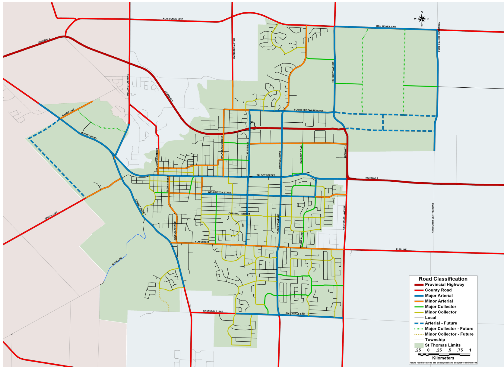
FIGURE ES.5 RECOMMENDED ROAD CLASSIFICATIONS
