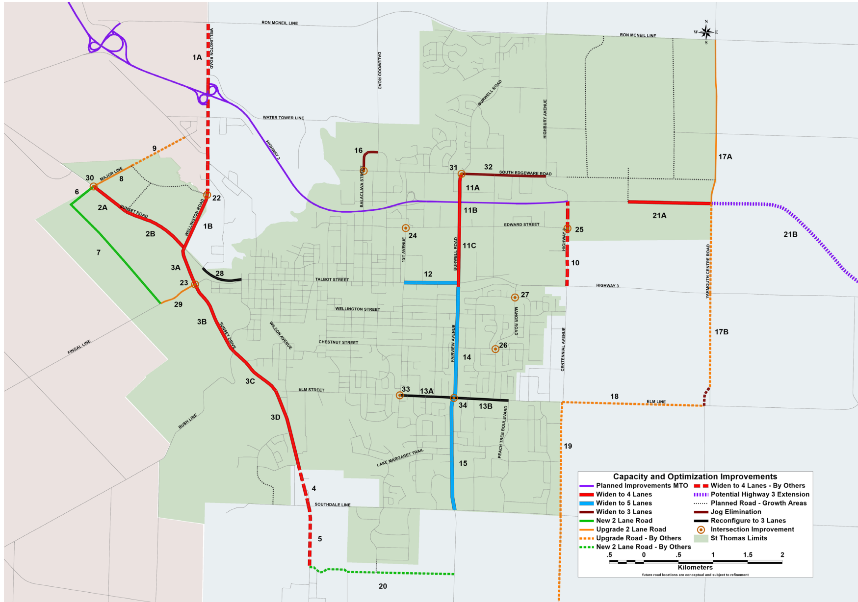
FIGURE ES.6 RECOMMENDED ROAD NETWORK IMPROVEMENTS
