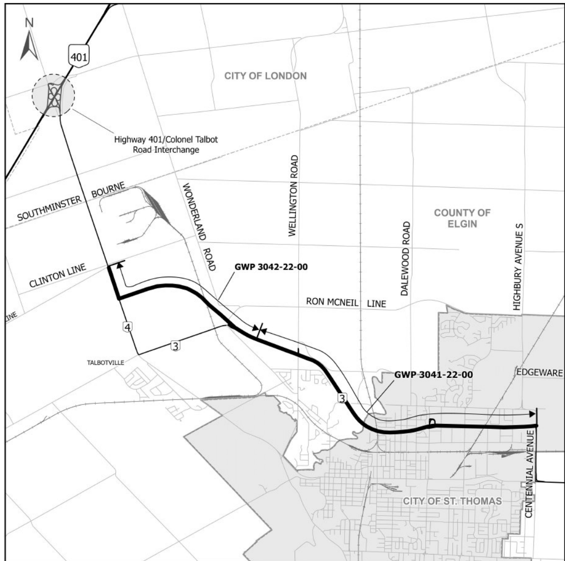
FIGURE 1.5: CURRENT / PLANNED MTO ROAD IMPROVEMENTS
