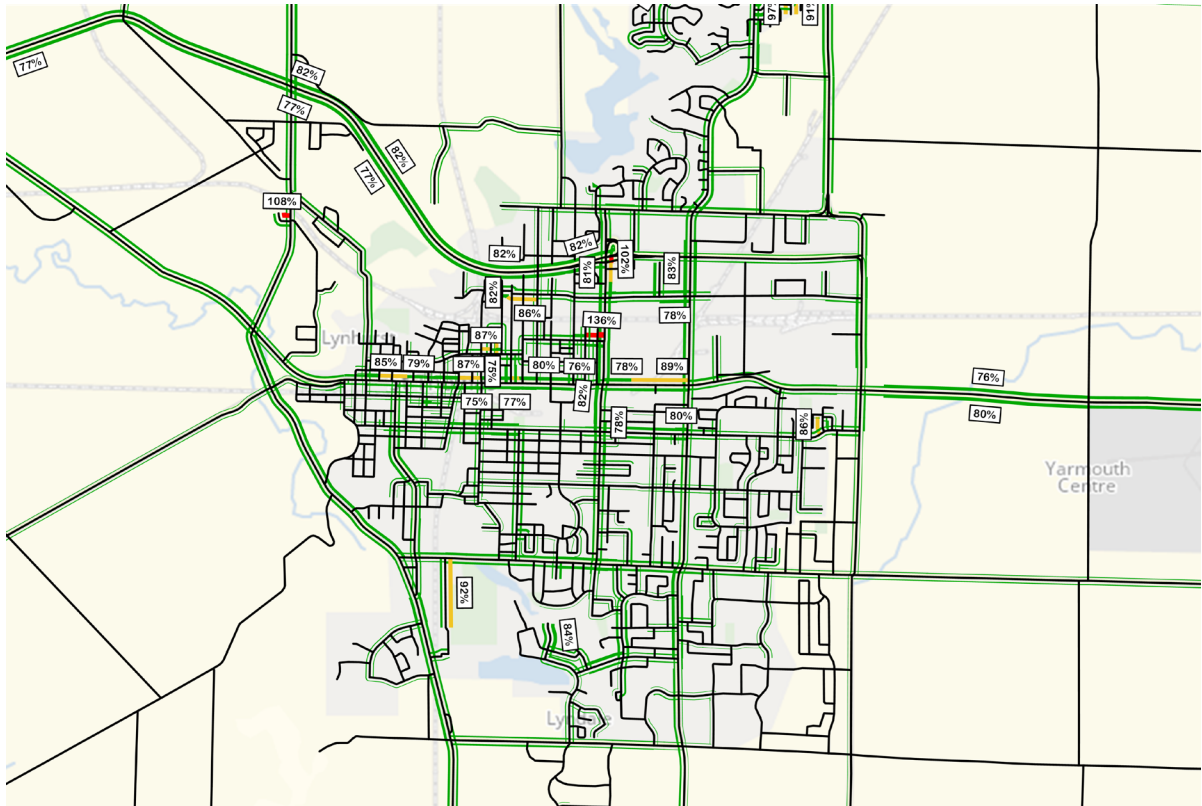
FIGURE 3.2: EXISTING ROAD NETWORK PERFORMANCE
