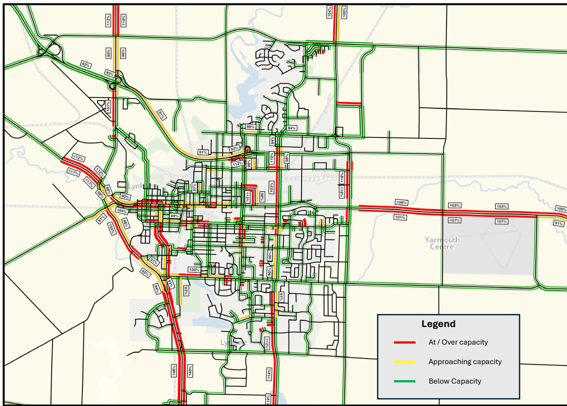
FIGURE 4.10: 2051 ROAD NETWORK DEFICIENCIES - ENHANCED TRANSIT
