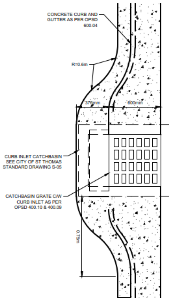
CURB INLET LAYOUT
