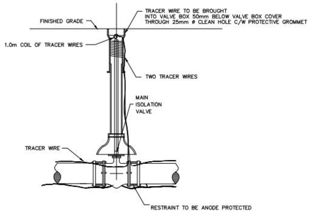
SCREW TYPE VALVE BOX
