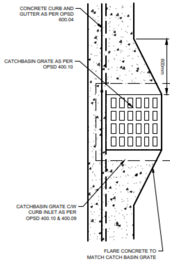
STD. CATCHBASIN LAYOUT
