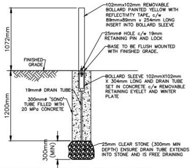
REMOVABLE BOLLARD DETAIL COMPONENTS AS SUPPLIED BY RUCKUS FENCE
